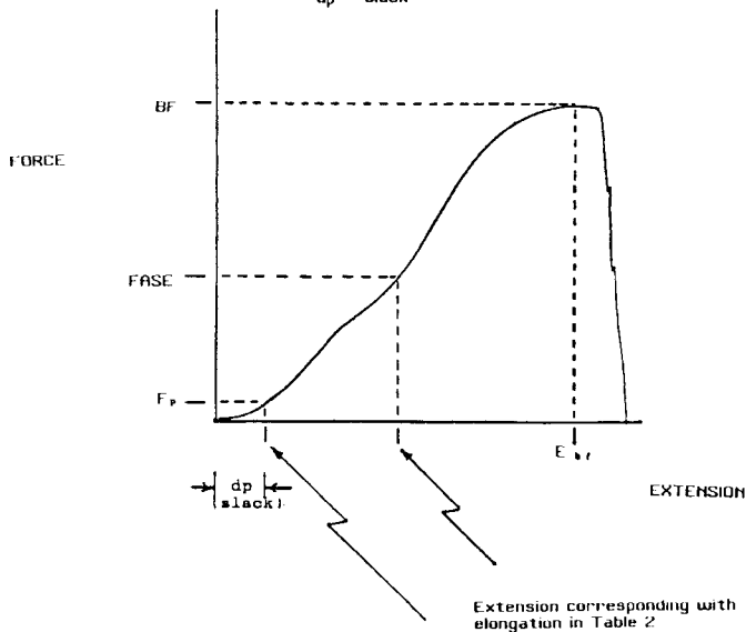
FIG. 1 Force-Extension Curve
