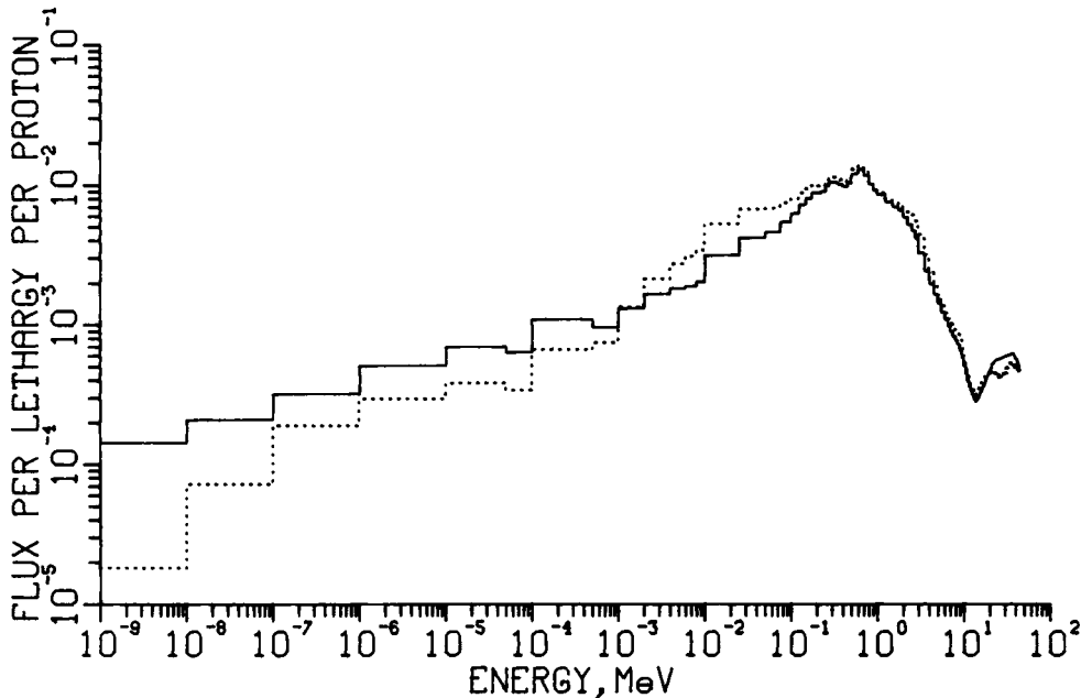
NOTE 1—Neutron flux spectrum at the Intense Pulsed Neutron Source of ANL with 500 MeV protons and a depleted uranium target. The solid line is calculated and the dashed is an adjusted spectrum based on radiometric dosimetry. (Data from Ref (12).)
