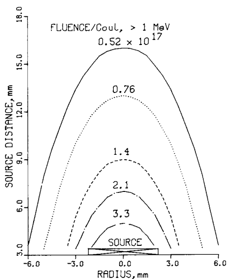
Note—Neutron fluence contours measured at the University of California with Davis Cyclotron Be(d,n), E_d = 30 MeV. (Data from Ref(10).)
