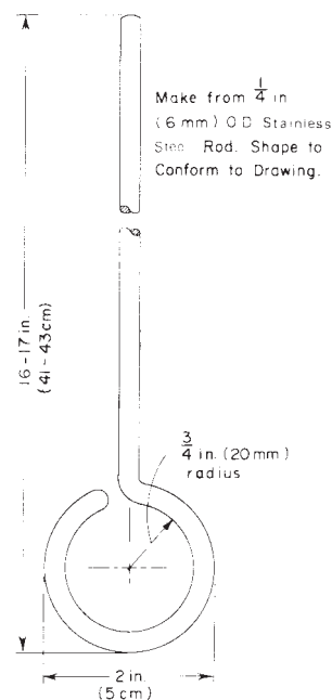
FIG. 6 Stirring Rod Detail
