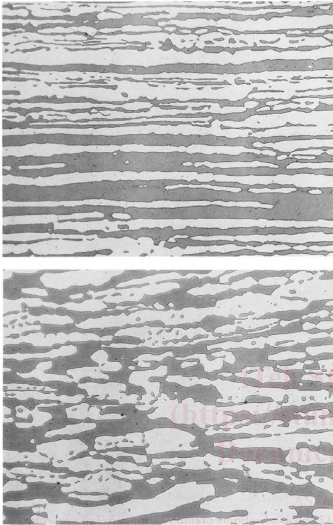
FIG. 1 Unaffected Structure in S31803: (a) Longitudinal Section and (b) Transverse Section (500× Magnification Before Reproduction)
