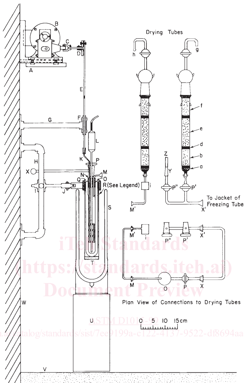
FIG. 1 Assembly of the Freezing-Point Apparatus (See preceding page for legend.) (continued)
