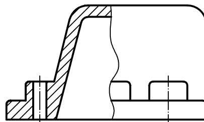
Figure 5 — Local cut
