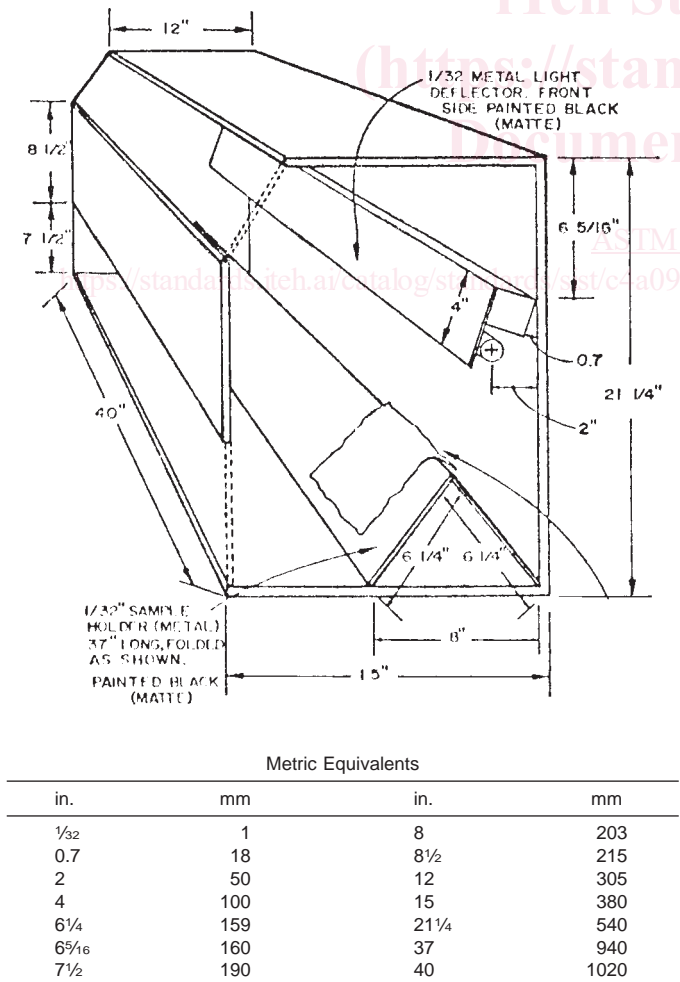
FIG. 5 Apparatus for Fabric Evaluation
