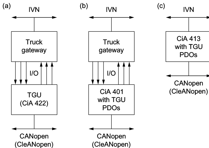
Figure 4 — Truck gateway implementation examples
