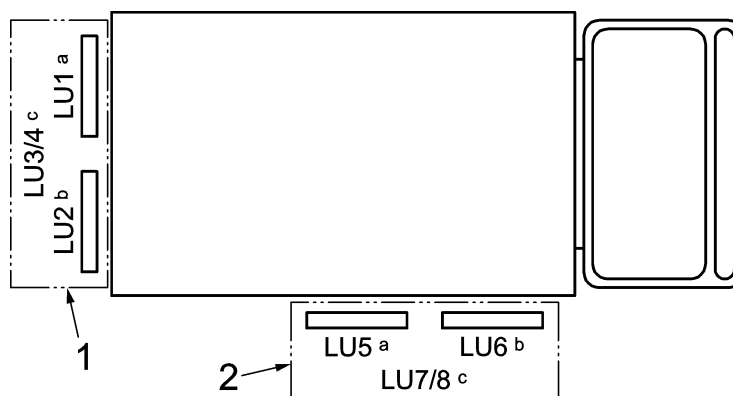
Figure 9 — LU numbering for the two compartment rear loader
