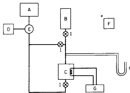
A—Vacuum Pump B—Test Gas Cylinders C—Gas Transmission Cell D—Vacuum Gage E—Trap F—Barometer G—Automatic Recorder (Optional) H—Mercury Manometer I—Needle Valve
