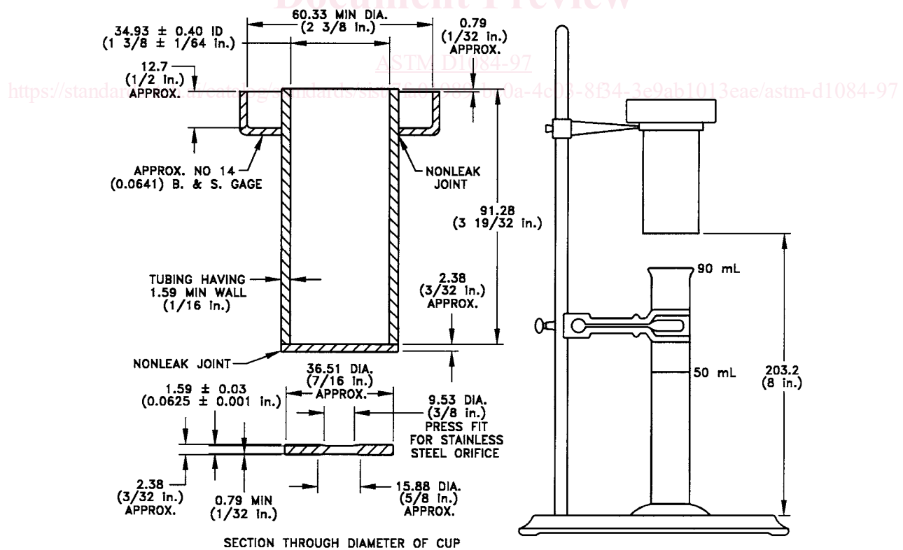
FIG. 1 Consistency Cups and Apparatus Assembly (Test Method A)
