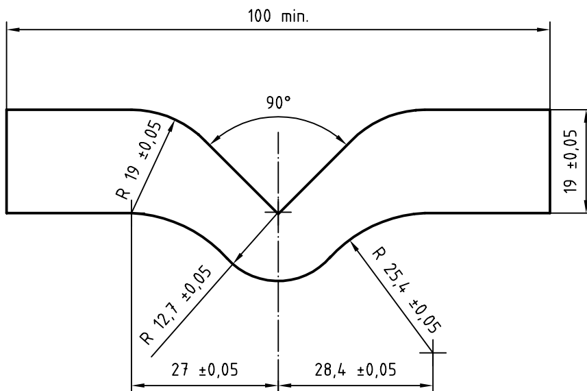
Figure 2 — Angle test piece die
