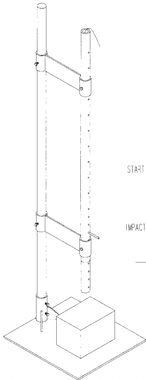
FIG. 2 Guided Free Fall
