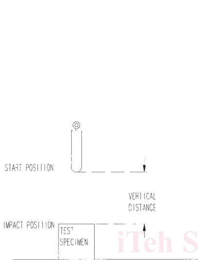
FIG. 1 Cylindrical Mass (steel rod)
