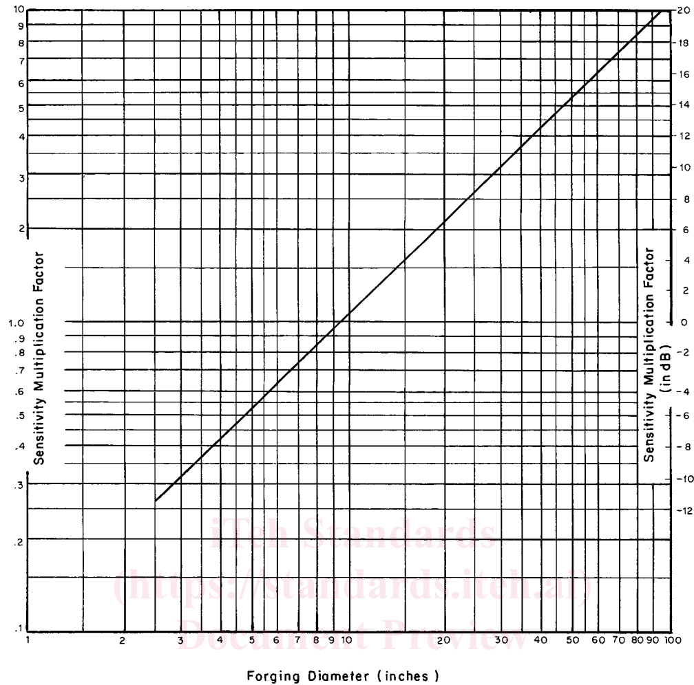
ASTM A 418-99(2003) SENSITIVITY MULTIPLICATION FACTORS FOR SOLID FORGINGS
