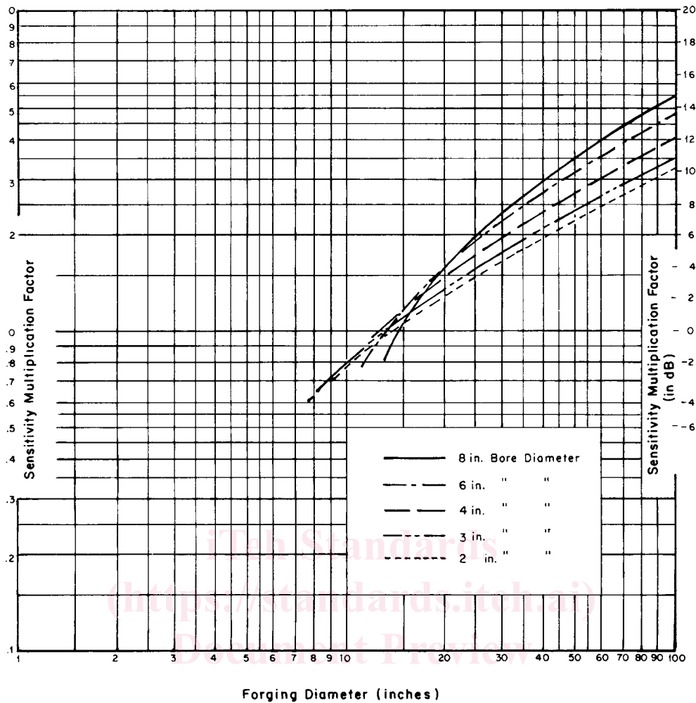
ASTM A 418-99(2003) SENSITIVITY MULTIPLICATION FACTORS FOR BORED FORGINGS
