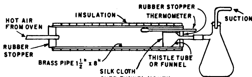
FIG. 1 Assembled Drier
