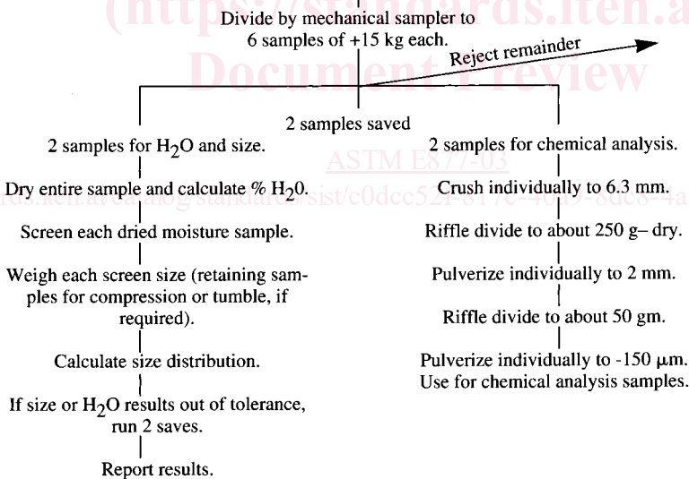
FIG. 3 Flowsheet Examples
