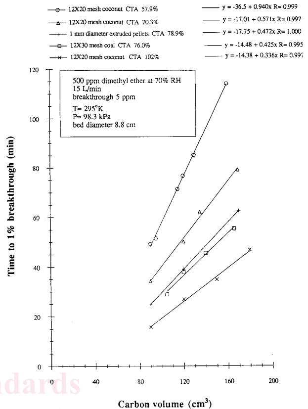
FIG. 3 Time to Breakthrough Versus Volume of Carbon
