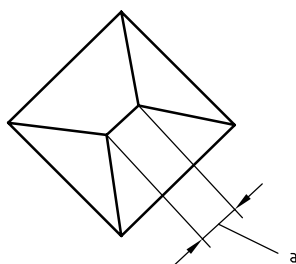
SIST ISO 4516:2004 https://standards.iteh.ai/standards/ISO/4516/2004/27e-4042-b42c-ba6ec42edc8c/sist-iso-4516-2004 Figure 1 — Vickers indenter
