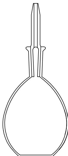
Figure 1 — Example of Gay-Lussac type pyknometer
