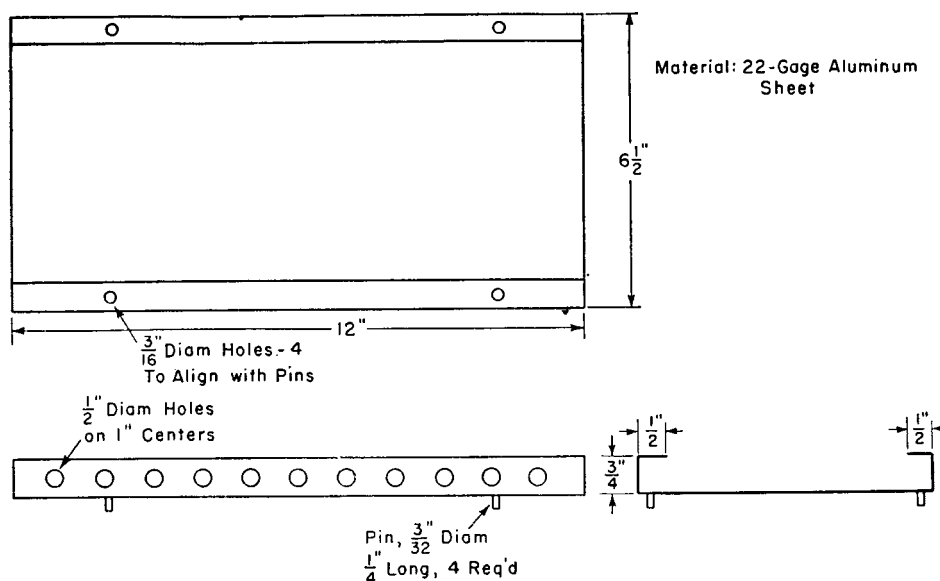
FIG. 1 Tray for 6 by 12-in. (150 by 300-mm) Foil
