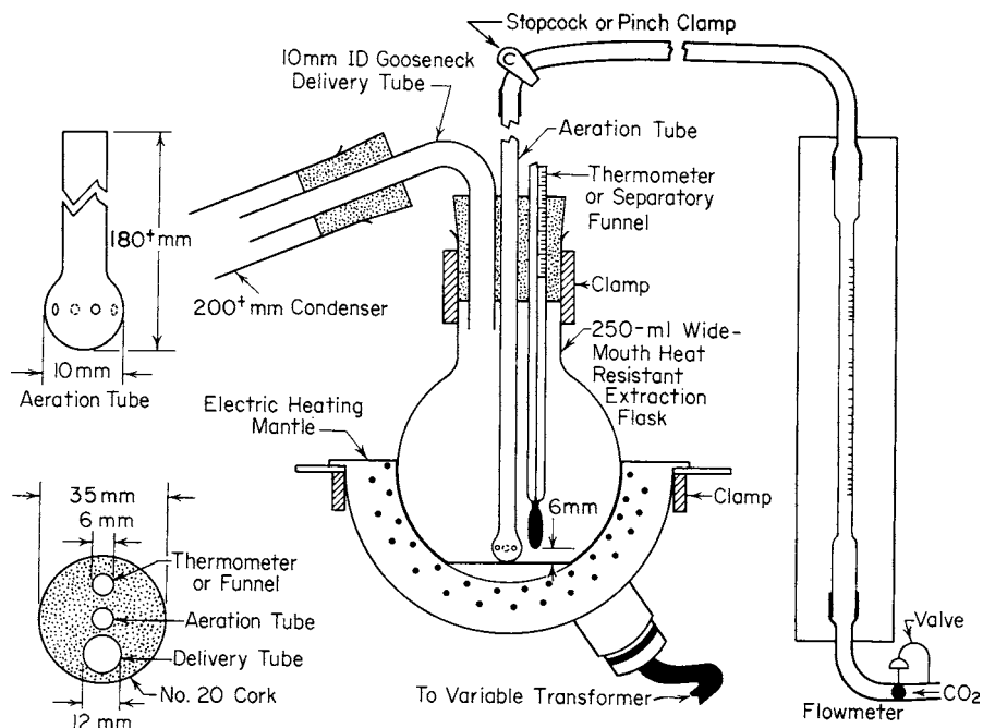
FIG. 1 Distillation Assembly for Bitumen Recovery
