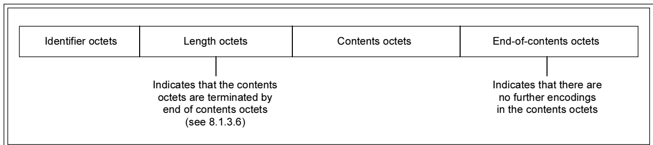
Figure 2 – An alternative constructed encoding
