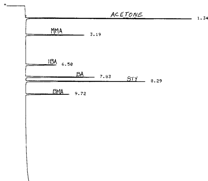
FIG. 1 Typical Chromatogram
