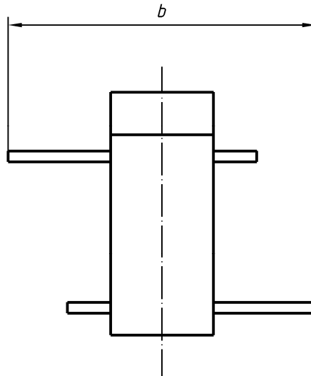
Figure 2 — Jacking width
