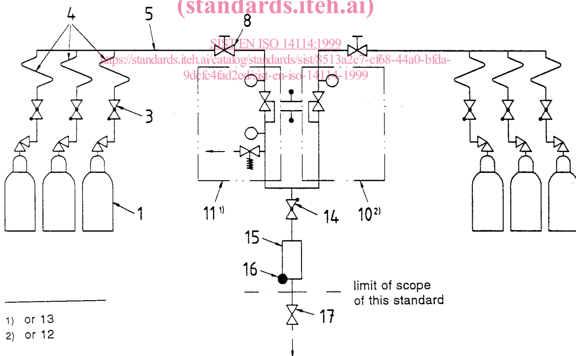
Figure A.2: System with three way valve and one regulator for up to 2 x 3 cylinders
