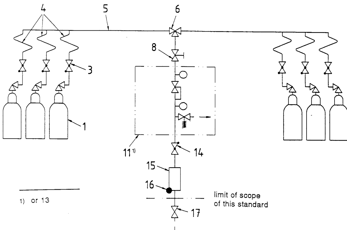
Figure A.2: System with three way valve and one regulator for up to 2 x 3 cylinders
