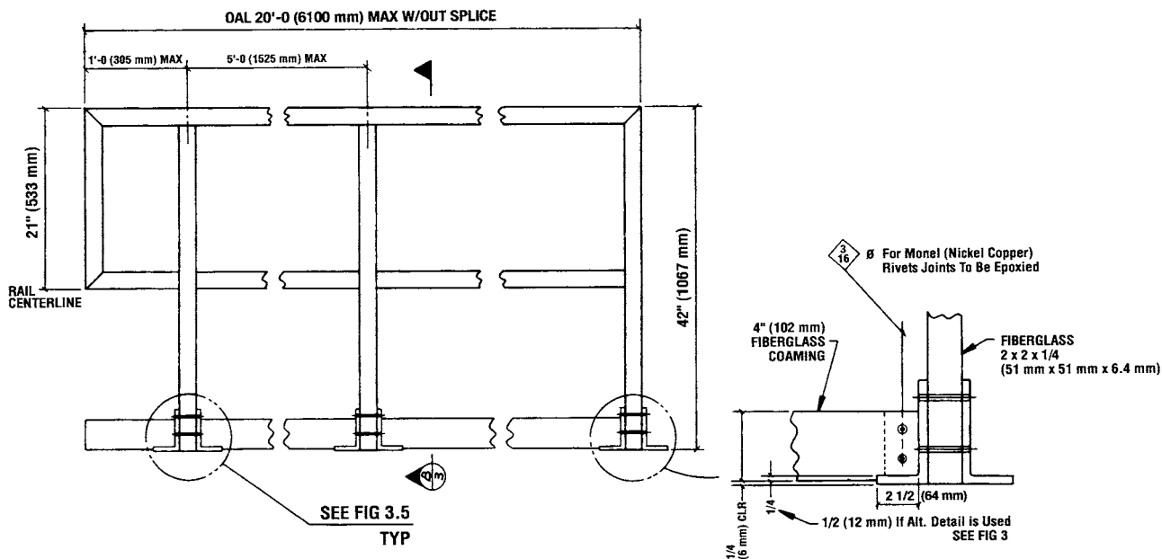
FIG. 1 Fiberglass Coaming
