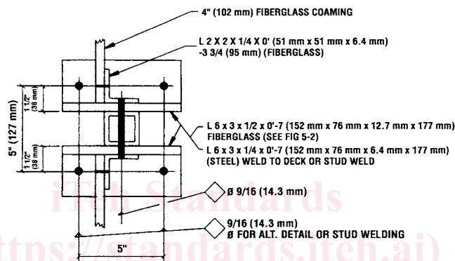
Welded to Steel Deck (Alternate—FRP Bolted to STL & Welded to Floor—SEE ALT DETAIL FIG 3)
