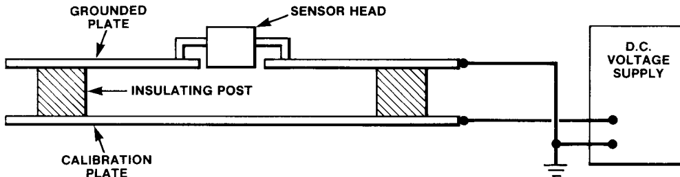
FIG. 5 Calibration Fixture
