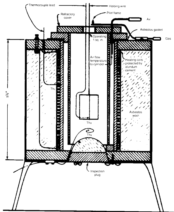
NOTE— Legend: Th 1 —Thermocouple on outer wall Th 2 —Thermocouple in air stream Th 3 —Thermocouple in or on the specimen
