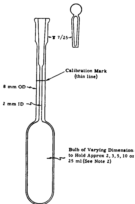
FIG. 1 Bingham-Type Pycnometer
