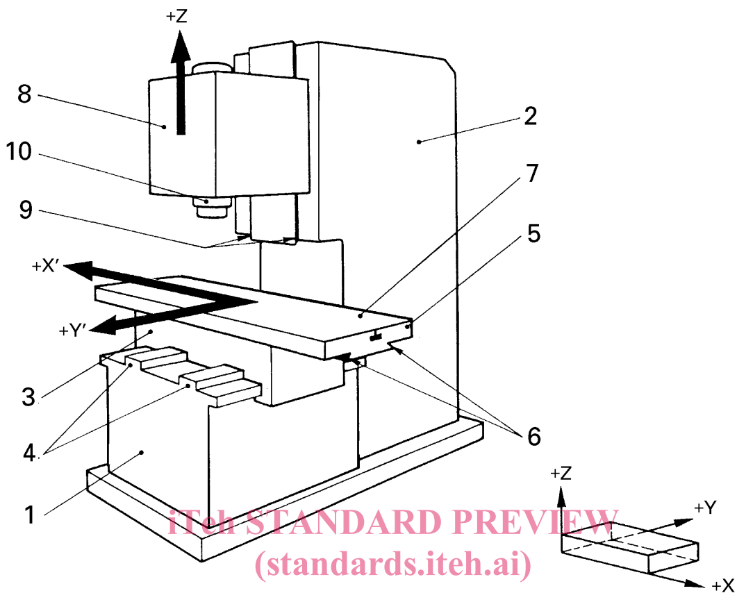
ISO 1984-2:2001 https://standards.iteh.ai/catalog/standards/sist/5b0680bc-5268-44a6-9f17-93da8636223c/iso-1984-2-2001 Figure 1 — Machines with vertical spindle
