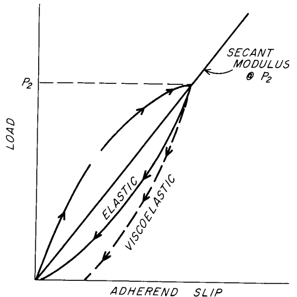
NOTE 1—The modulus is represented by the secant modulus line at some load P_2 less than the load to cause failure. FIG. 2 Load-Slip Diagram of Nonlinear Adhesive Under Cyclic Low-Level Loading Showing Both Elastic and Viscoelastic Recovering Diagrams
