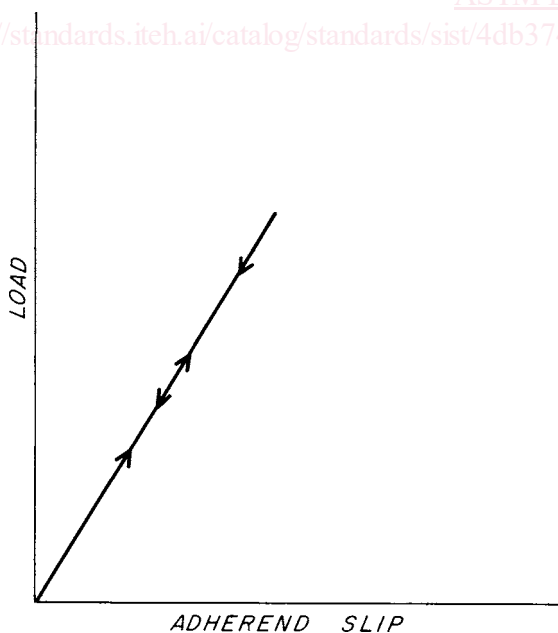
NOTE 1—Case load and unload diagrams and modulus line are congruent. FIG. 1 Load-Slip Diagram of Linear Elastic Adhesive Under Cyclic Low-Level Loading
