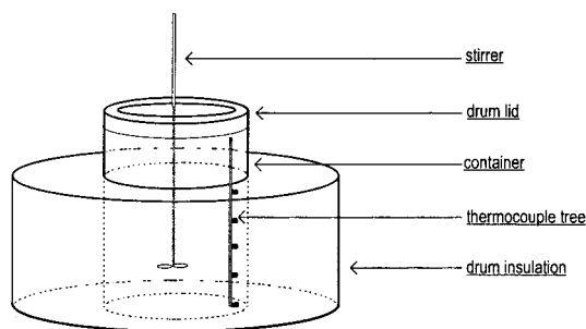
FIG. 1 Water-Bath Calorimeter
