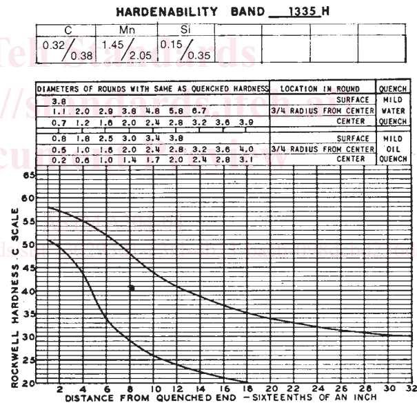
NOTE—1 in. = 25.4 mm. FIG. 3 Limits for Hardenability Band 1335 H
