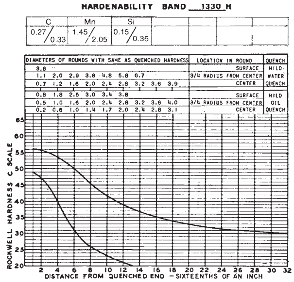
NOTE—1 in. = 25.4 mm. FIG. 2 Limits for Hardenability Band 1330 H
