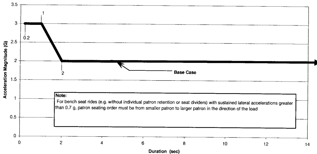
FIG. 7 Time Duration Limits for ±Gy (Eyes Left or Eyes Right)
