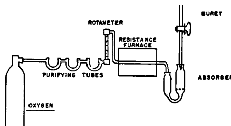
FIG. 3 Schematic Illustration of Resistance-Type Furnace
