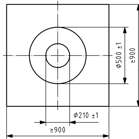
Figure 1 — Baseplate iTeh STANDARD PREVIEW (standards.iteh.ai)
