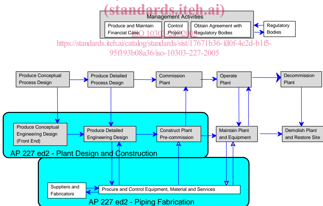
Figure 2 — Process plant life cycle activity coverage
