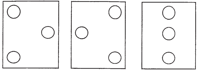
Specimen 1 Specimen 2 Specimen 3 FIG. 3 Impact Locations for Small Missile Test (Each Type of Infill)
