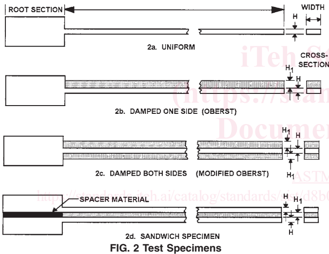
FIG. 2 Test Specimens
