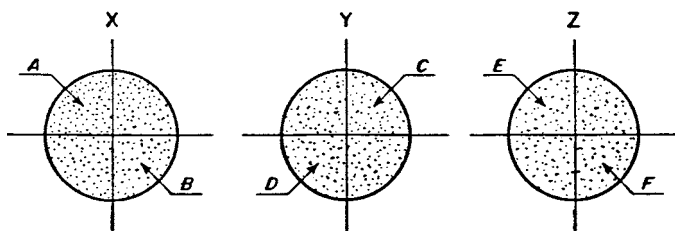
FIG. 2 Quartering Samples
