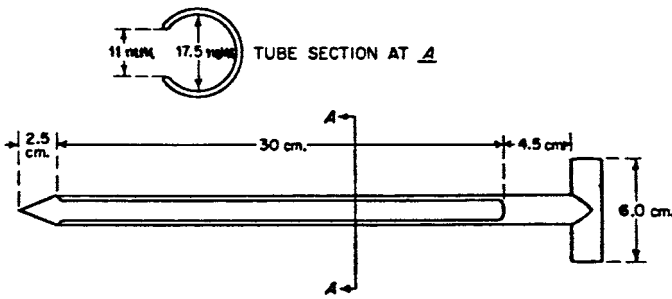
FIG. 1 Sampling Tool
