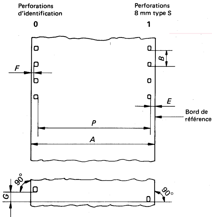
FIGURE 2 – Film perforé 1-0
