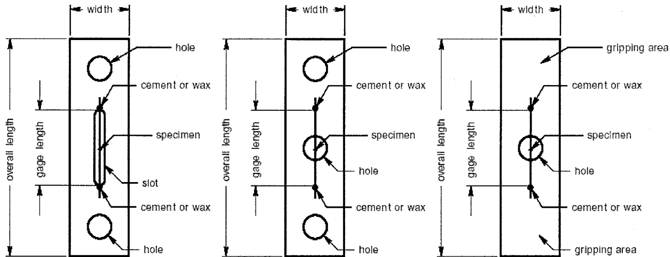
FIG. 3 Mounting Tab
