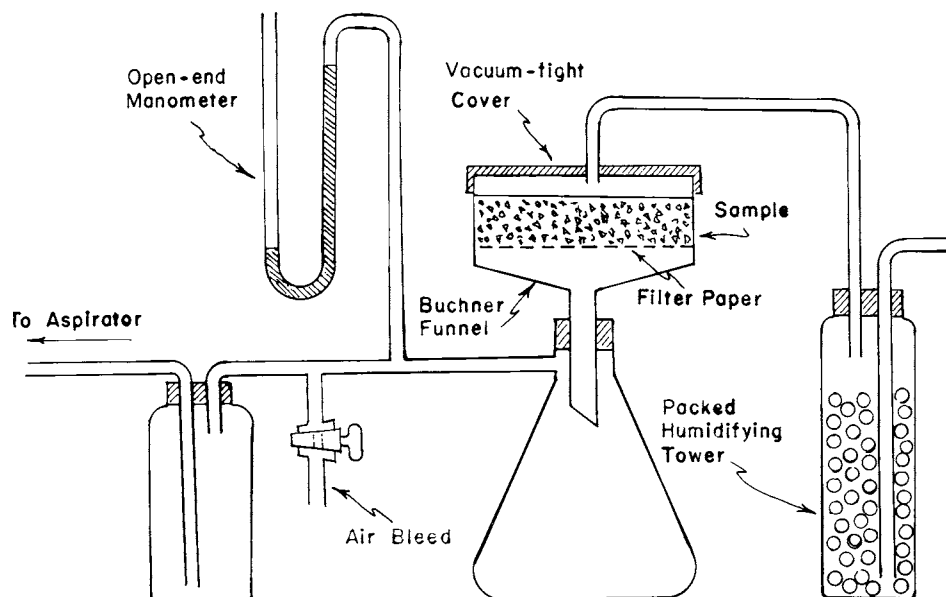
FIG. 2 Typical Arrangement of Water-Draining Apparatus
