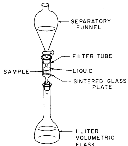
FIG. 3 Typical Arrangement of Apparatus for Salt-Splitting Capacity
