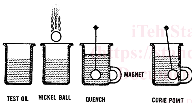
FIG. 2 Test Sequence in Beaker
