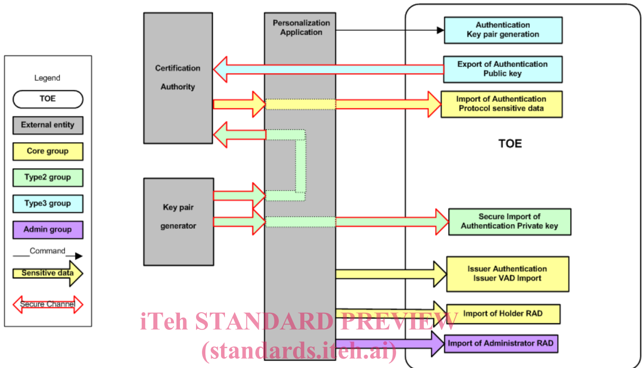
SIST EN 419251-1:2013 https://standards.iteh.ai/catalog/standards/sist/506095c-407d-4a90-889d-d7d664fc94d6/sist-en-419251-1-2013 Figure 2 — Personalisation application environment
