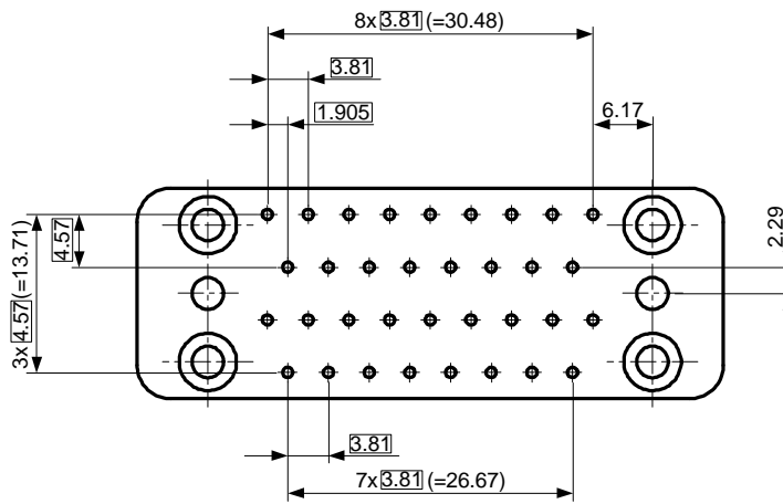
Figure 3 – Contact spacing dimensions
