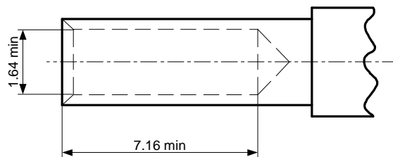
Figure 5 – Female contact
