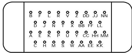
DCE contact arrangement viewed from connector front (DTE side)
