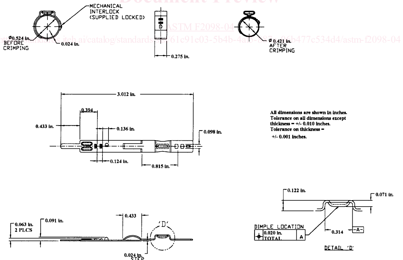
FIG. 1 Stainless Steel Clamp Dimensions, 3/8-in. nominal
