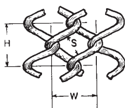
FIG. 1 Mesh Dimensions for ⅝-in., ½-in., and ⅜-in. Fabric
