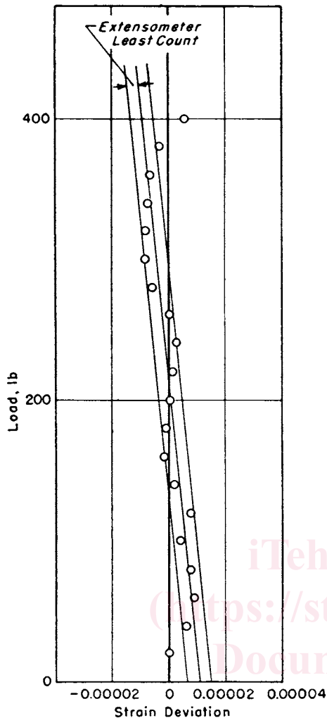
FIG. 2 Load-Deviation Graph
