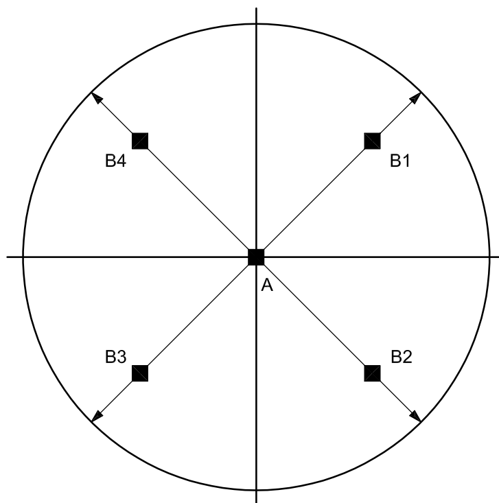
iTeh STANDARD PREVIEW Figure 1 — Image points to be tested for optical resolution (standards.iteh.ai)
