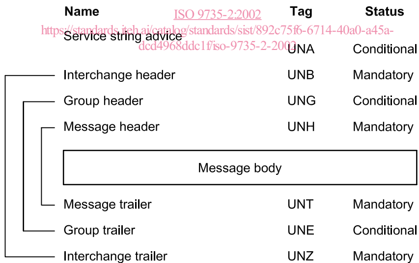
Figure 1 — Batch EDI interchange structure
